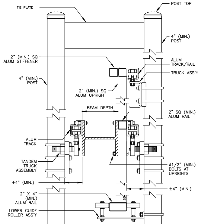
SECTION NOT TO SCALE
